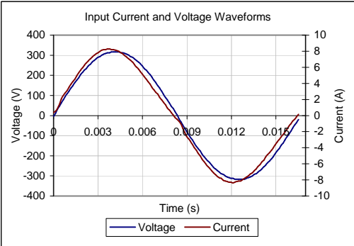
Input AC Current Waveform (ITHD = 5.3%, 100% Load)
